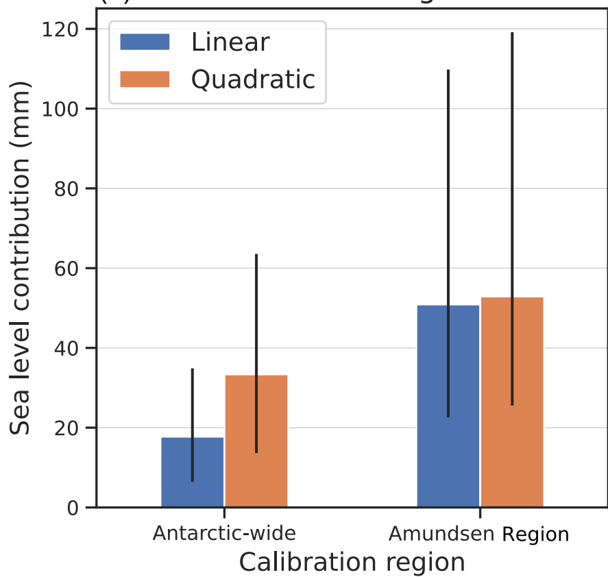
(b) Amundsen region
