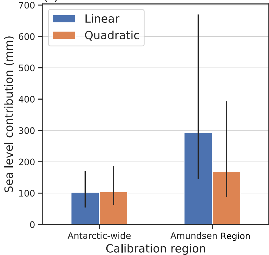
(a) Antarctic Ice Sheet
