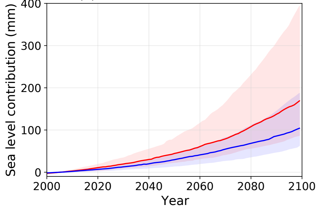
(a) Antarctic Ice Sheet: SSP5-8.5
