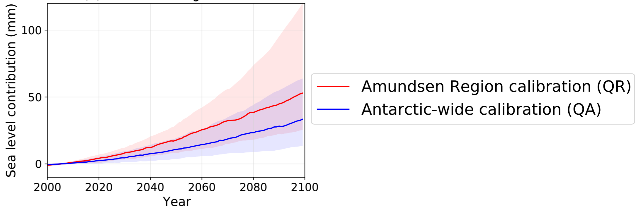
(b) Amundsen Region: SSP5-8.5
