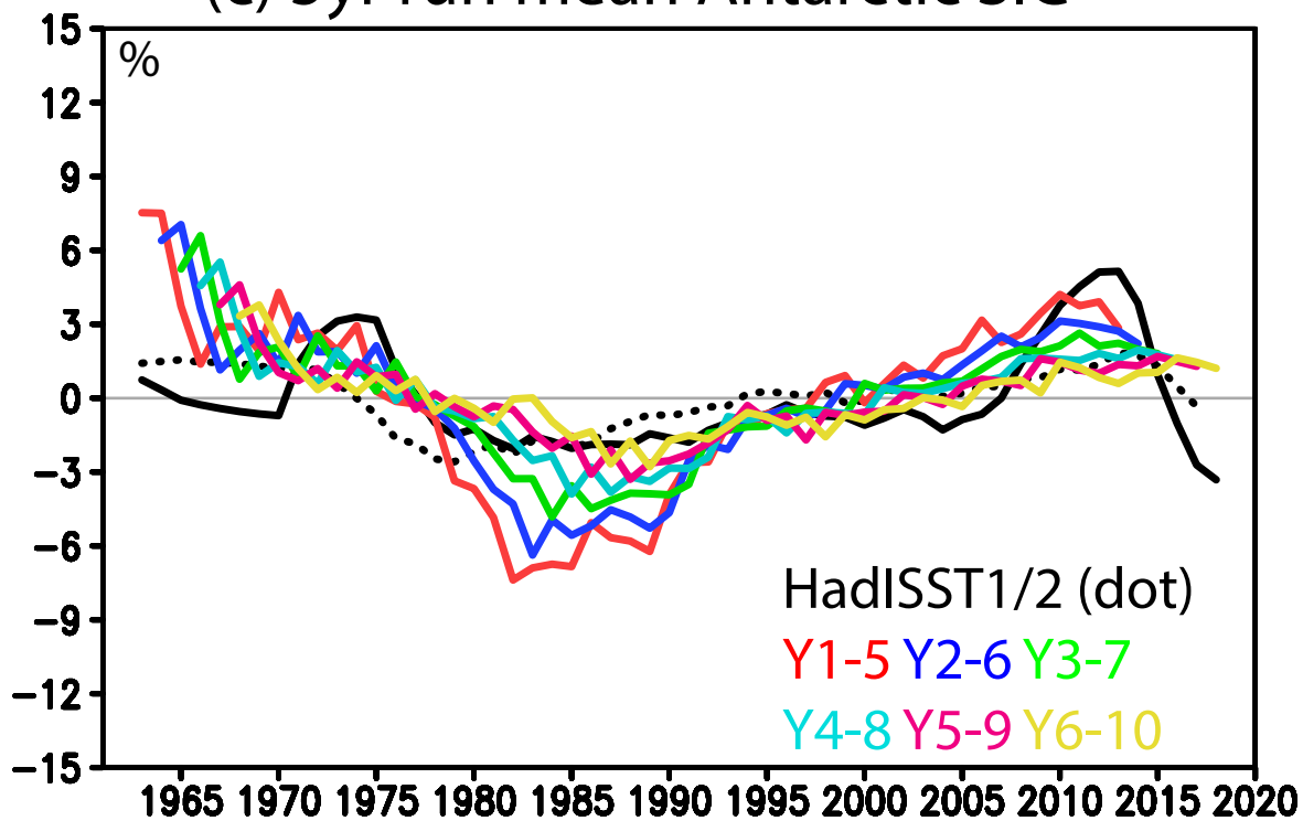
(c) 5yr run mean Antarctic SIC
