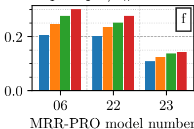
Surf. precip. / # time steps
