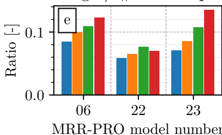
Virga / # time steps
