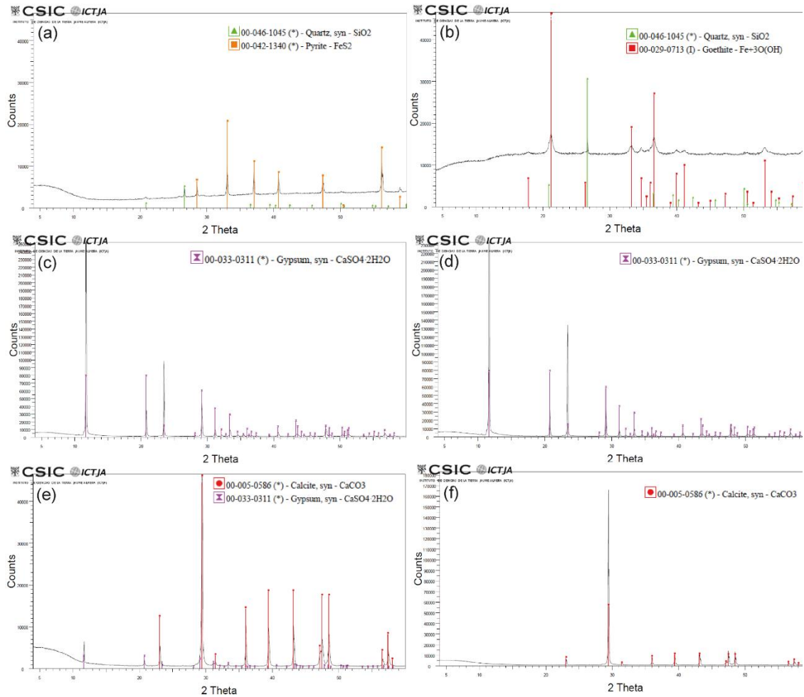
Fig. S1. X-ray diffraction analyses. (a) and (b) pyrite and goethite from the limestone host rock. (c) and (d) Cryogenic gypsum crystals from room D. (e) Cryogenic calcite and gypsum from room G. (f) Cryogenic cave calcite from room K.
