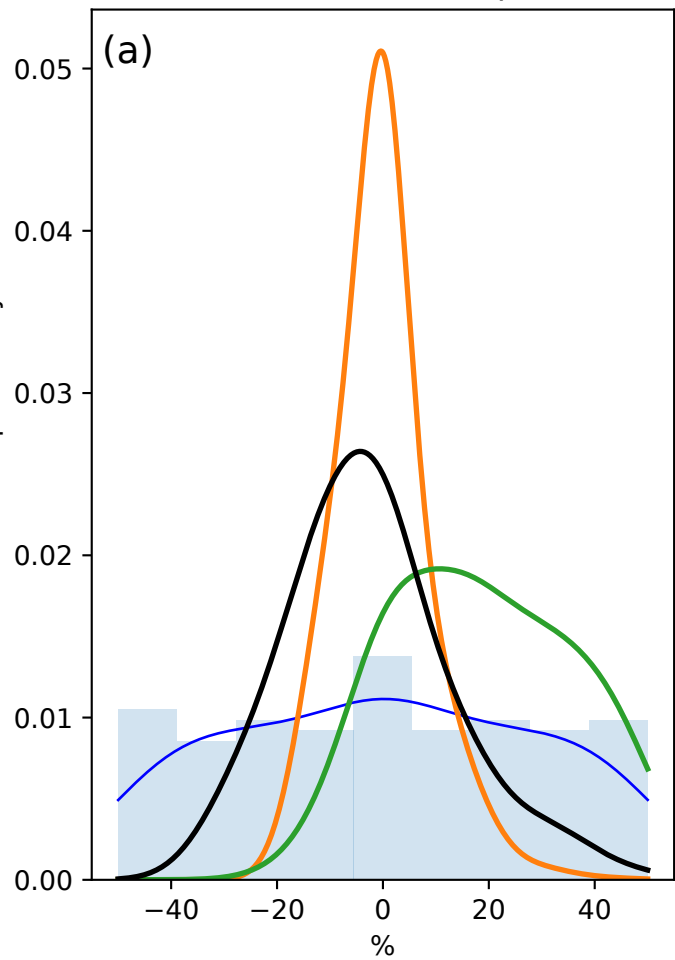
basal friction multiplier
