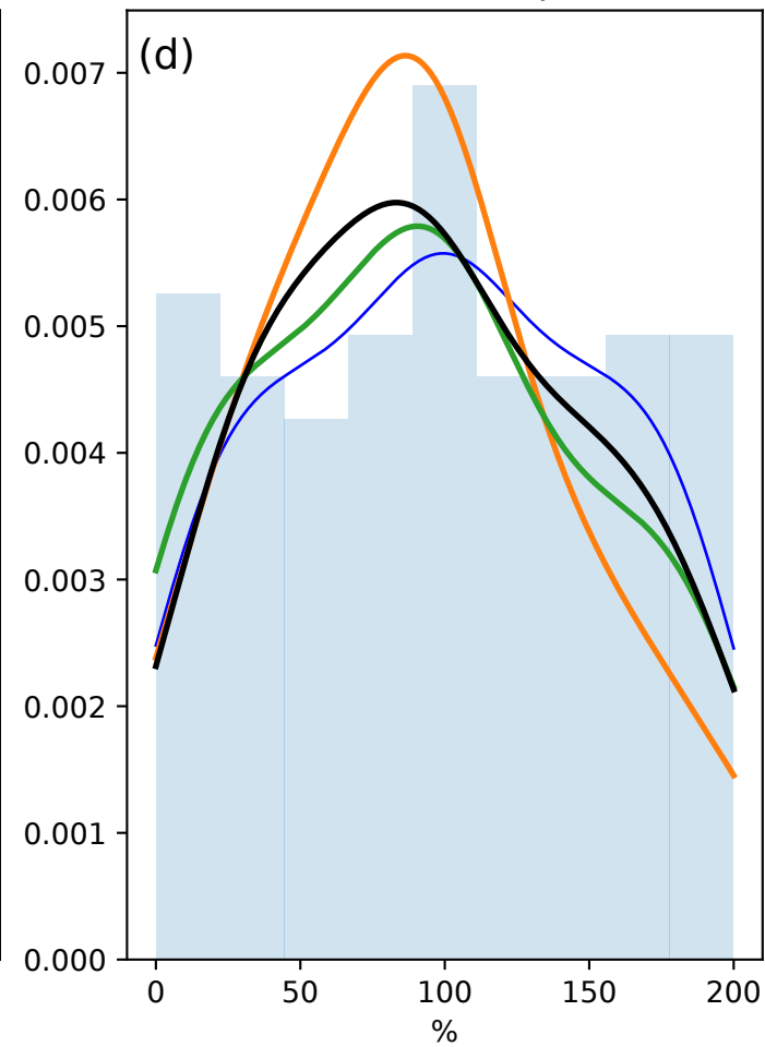
SMB seasonal amplitude
