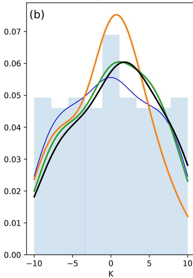
ice temperature shift
