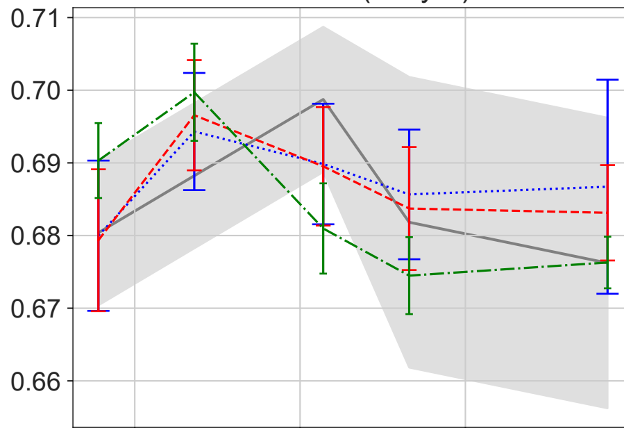
Cluster 4 (2-layer)
