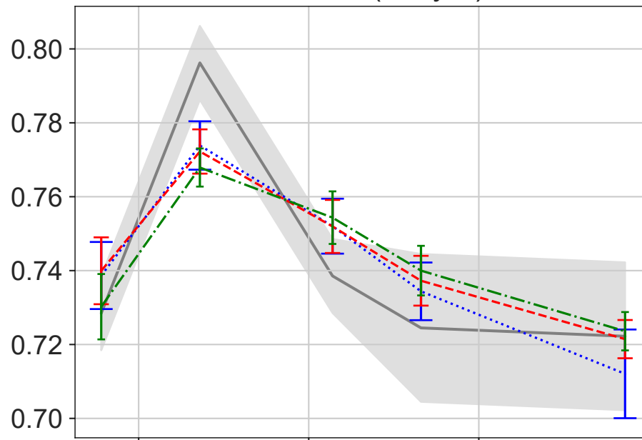
Cluster 7 (2-layer)
