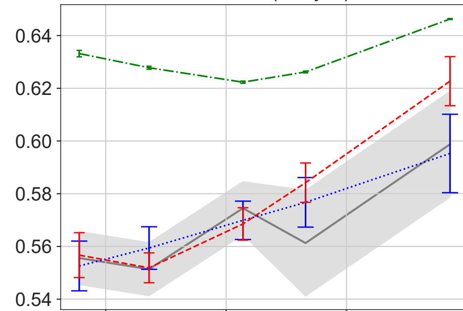
Cluster 2 (2-layer)
