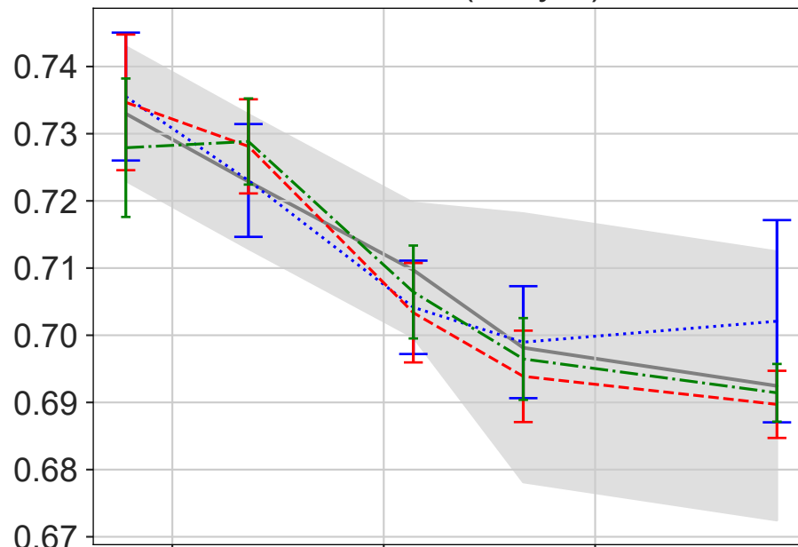
Cluster 1 (2-layer)
