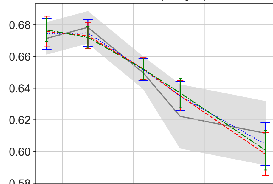
Cluster 5 (3-layer)
