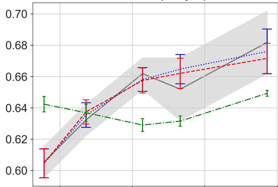
Cluster 0 (2-layer)
