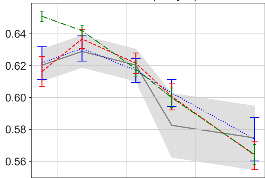
Cluster 3 (3-layer)
