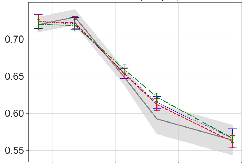
Cluster 6 (3-layer)
