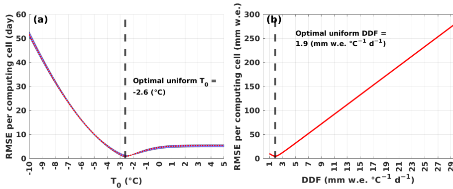
Figure C1. (a) Dotted red curve is the average of the RMSE across all satellites along each uni-PDD T_0 experiment. In each uni-PDD T_0 experiment, we calculate the RMSE between the time series of the annual sum of melt days over all computing cells between the uni-PDD model and each satellite estimate. Blue envelope covers the span of the three individual satellite results. Vertical dashed black line marks the optimal uni-PDD T_0 suggested by the minimal RMSE. (b) Red curve is the RMSE along each uni-PDD DDF experiment. In each uni-PDD DDF experiment, we calculate the RMSE between the time series of the annual sum of melt amount over all computing cells between the uni-PDD model and RACMO2.3p2. Vertical dashed black line marks the optimal uni-PDD DDF suggested by the minimal RMSE.
