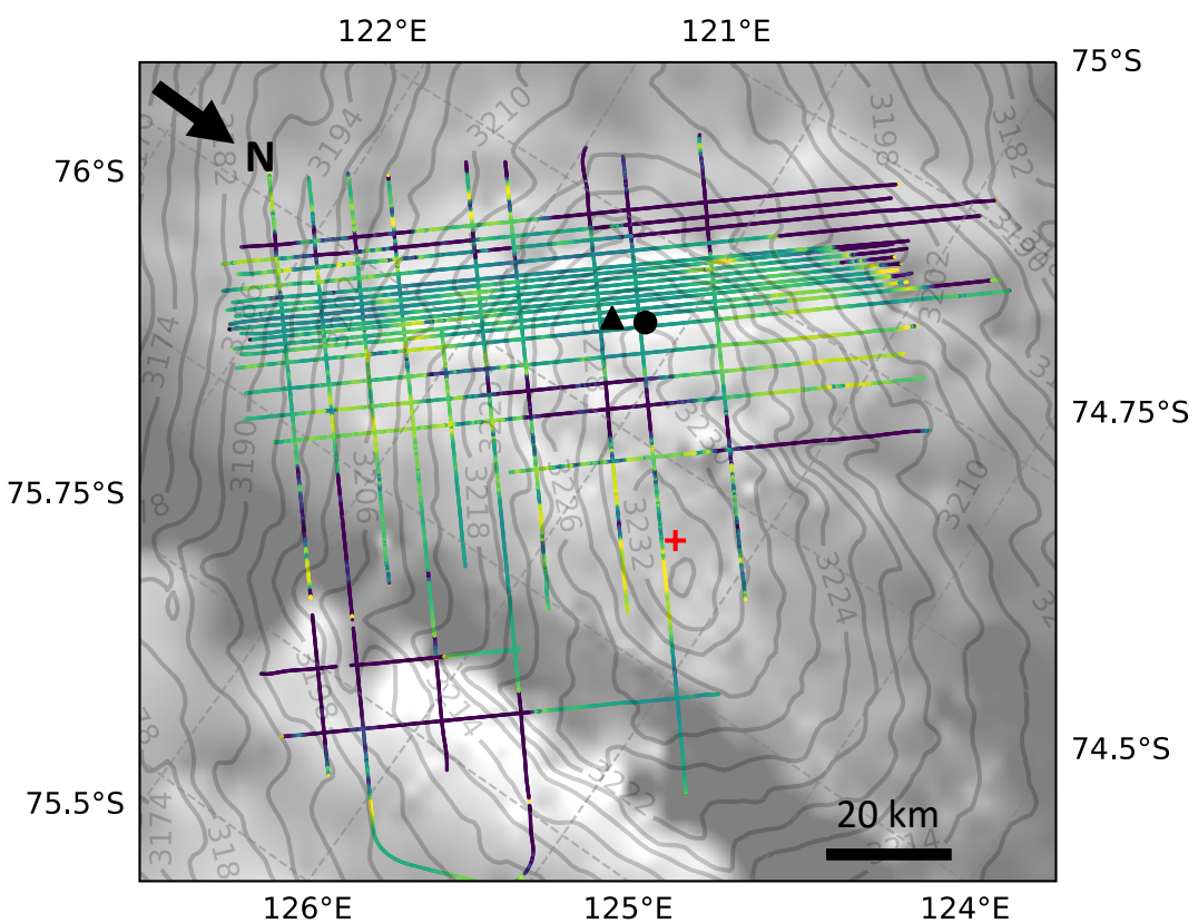
(a) Dome C - HiCARS
