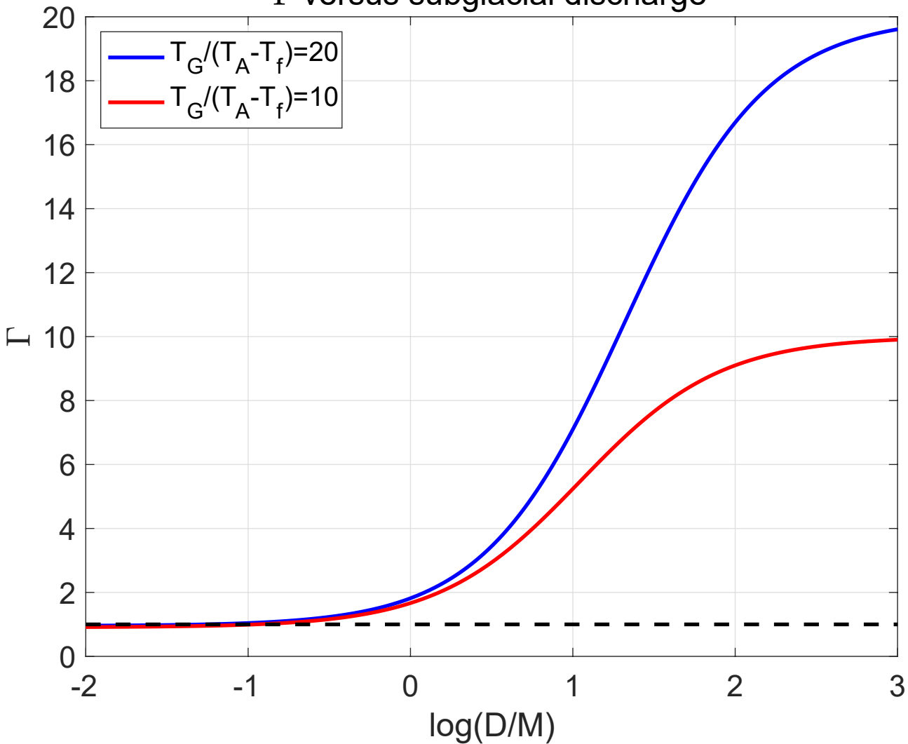
\Gamma versus subglacial discharge
