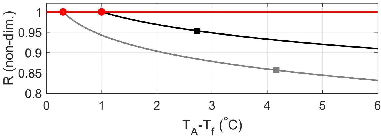
(b) R Factor versus T_A - T_f
