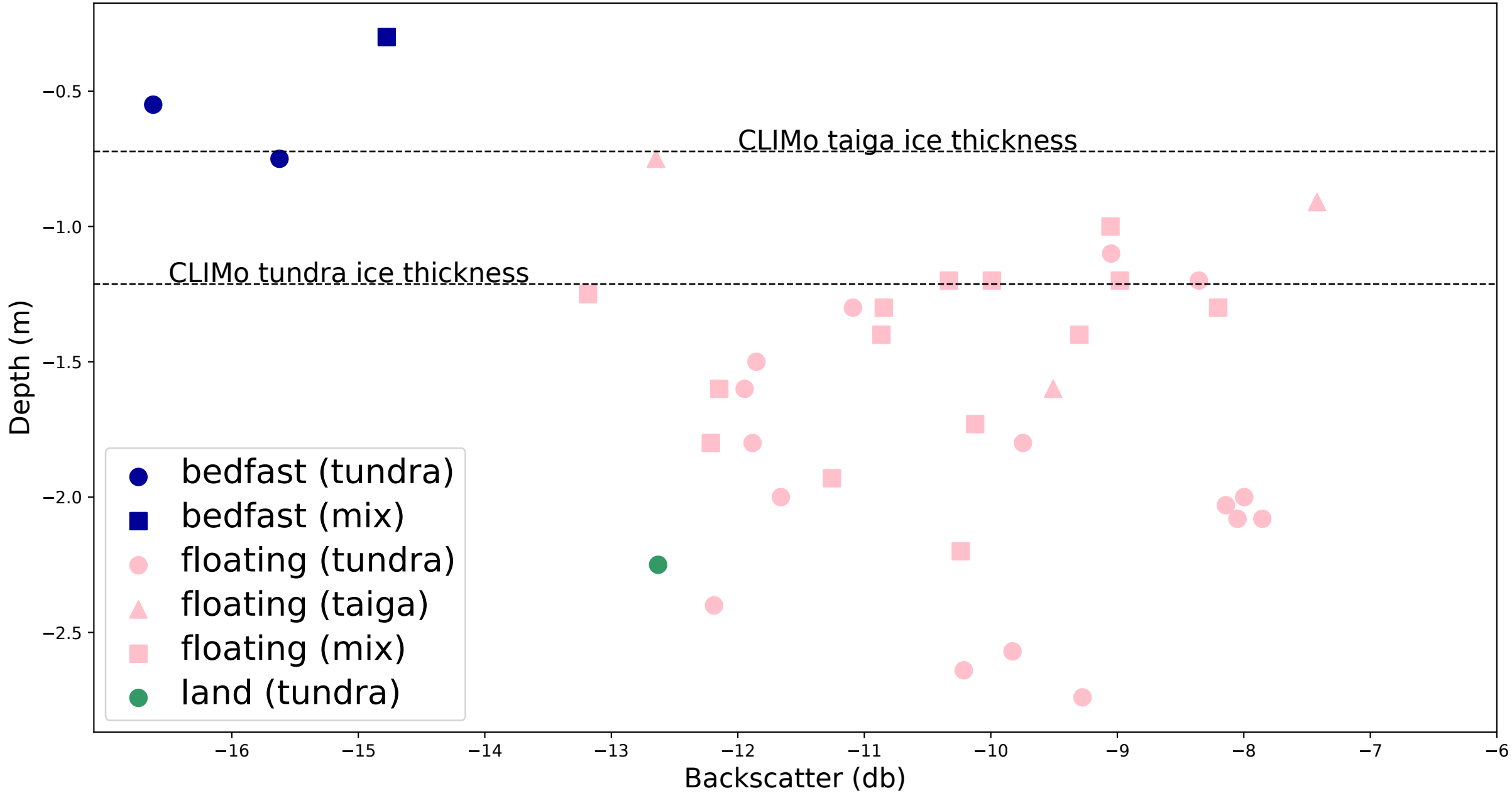
Field Measurements (summer 2000) of Lake Depth vs. TempCNN output (spring 2000)
