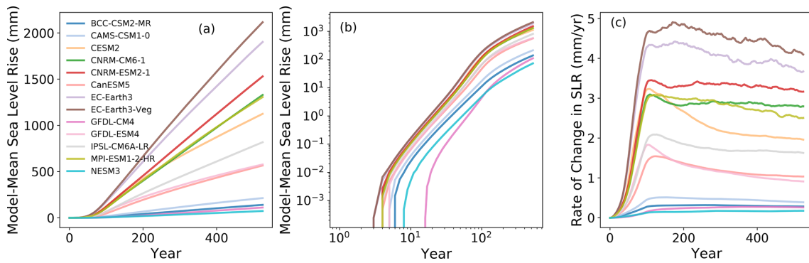
Figure A3. (a) Model-mean sea level rise, (b) model-mean sea level rise on log–log scale and (c) model-mean SLR rate of change ( \text{mm yr}^{-1} ).
