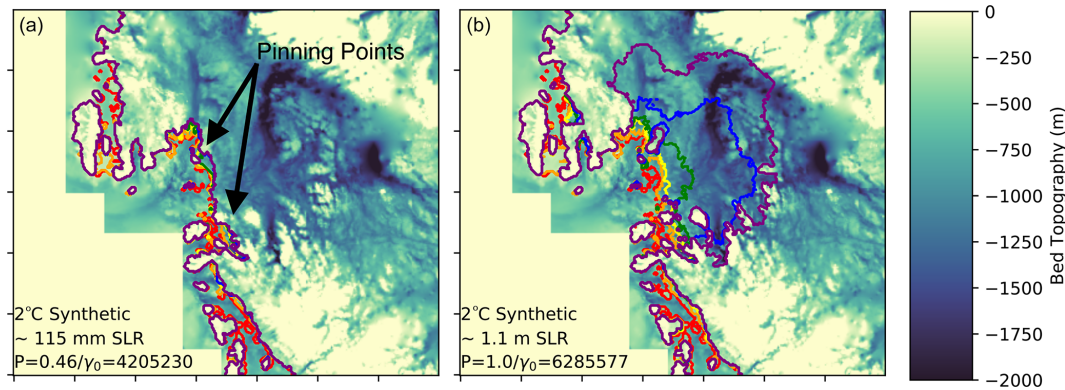
Figure 14. Grounding line location evolution over the 2°C synthetic run for (a) p = 0.46/\gamma_0 = 4205230 and (b) p = 1.0/\gamma_0 = 6285577 . Red, orange, yellow, green, blue and purple contours indicate years 0 to 525 at roughly 100-year intervals. Shaded background shows sea floor topography (m). Negative values indicate below sea level. Note that the ice in this area is largely grounded below sea level.
