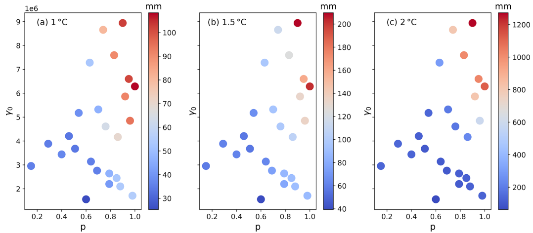
Figure A9. Final (500 years) sea level contribution from the Amundsen under three different synthetic forcing scenarios as a function of \gamma_0 versus p . The panels correspond to the three experiments: 1 °C (a), 1.5 °C (b) and 2 °C (c). Note the different color-bar scales.
