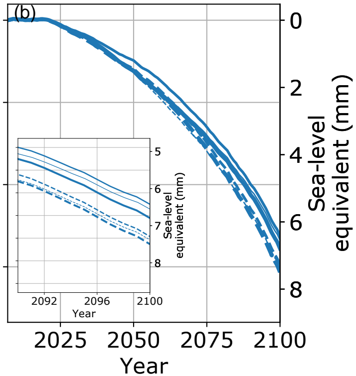
CNRM-CM6
