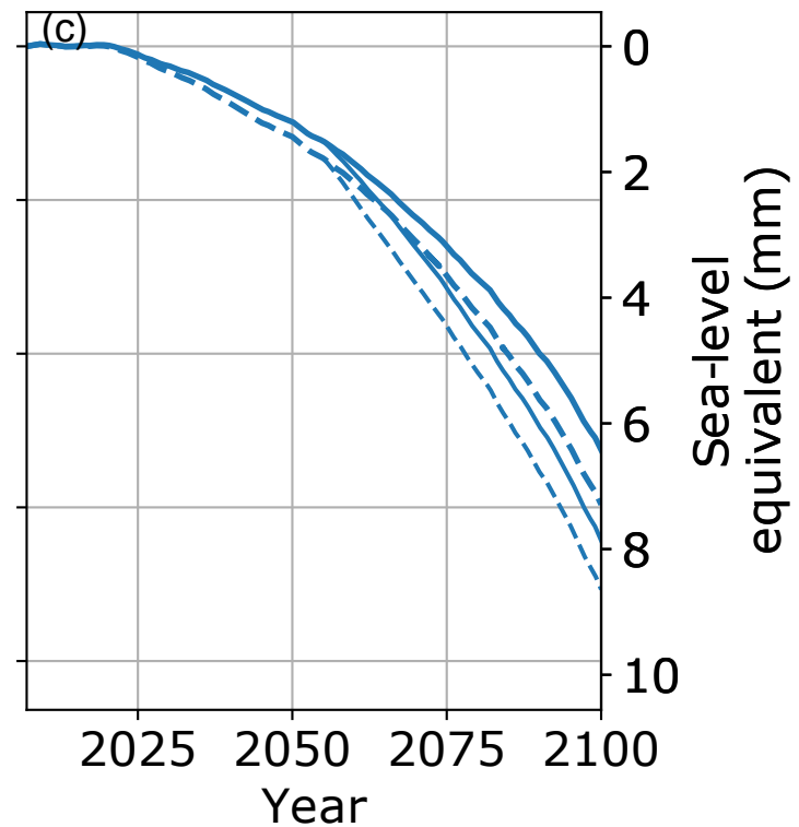
CNRM-CM6
