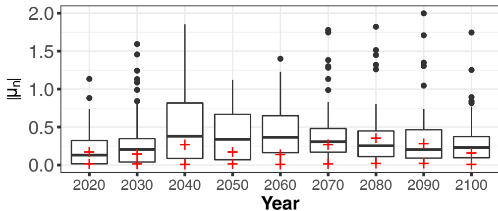
(g) IceFlow
