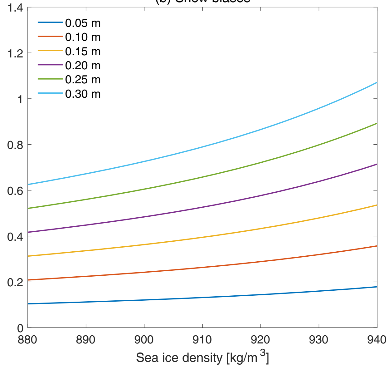
(b) Snow biases
