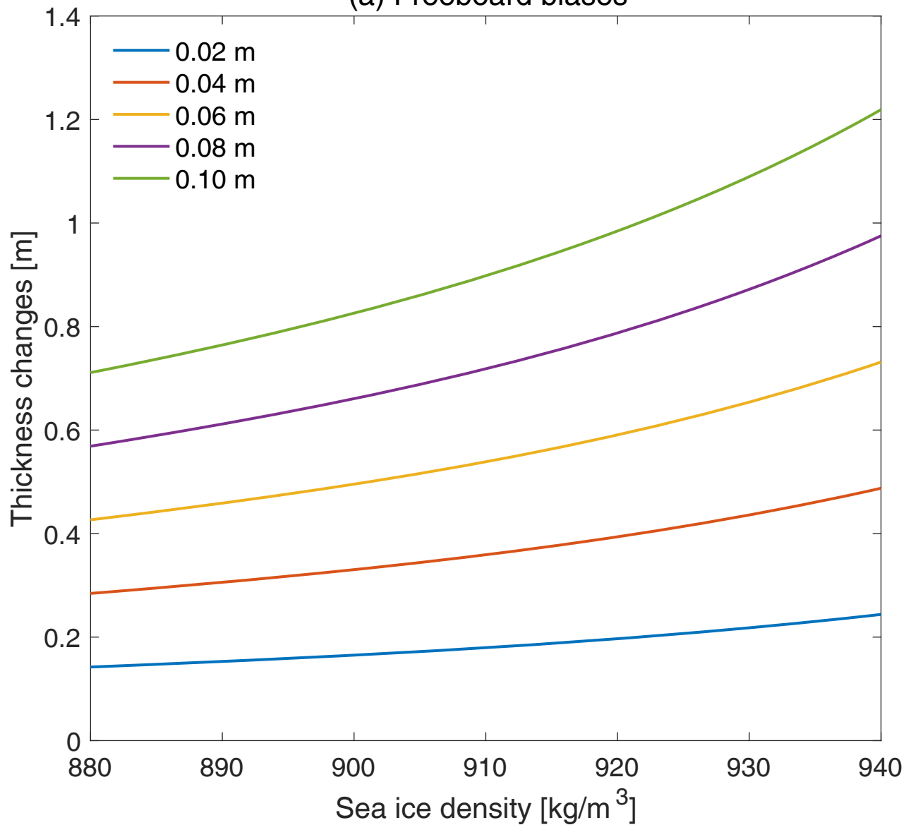
(a) Freeboard biases
