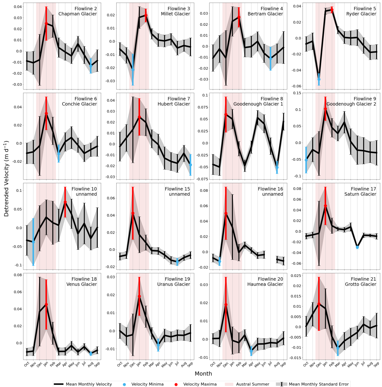
Figure 5. Detrended SAR-derived observations of mean monthly ice flow between 2014 and 2020 (black) and associated mean monthly standard error (grey shading). Observations are averaged across the 10 km 2 dashed boxes shown in Fig. 1. Blue and red error bounds denote velocity minima and maxima, respectively. Translucent red shading denotes the timing of austral summertime (December–February, inclusive). Note that the y-axis limits vary between panels.
