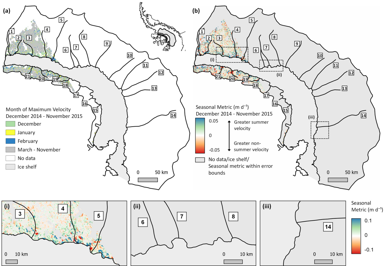
Figure B1. Same as Fig. 3 but showing spatially resolved patterns of seasonal ice flow as observed between December 2014 and November 2015. Panels (a) shows the month of maximum velocity ( v_{ime} ) and (b) the calculated velocity anomaly ( v_{anomSAR} ). In (b), positive velocity anomalies (blue) indicate summertime speed-up and negative (red) greater velocity during non-summertime months. Dashed boxes denote the location of the inset boxes (i–iii). Note that insets ii and iii contain no data for the period December 2014–November 2015. See also Figs. B2–B4.
