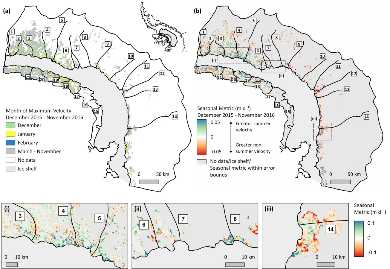
Figure B2. Same as Fig. 3 but showing spatially resolved patterns of seasonal ice flow as observed between December 2015 and November 2016. Panel (a) shows the month of maximum velocity ( v_{\text{time}} ) and (b) the calculated velocity anomaly ( v_{\text{anomSAR}} ). In (b), positive velocity anomalies (blue) indicate summertime speed-up and negative (red) greater velocity during non-summertime months. Dashed boxes denote the location of the inset boxes (i–iii). See also Figs. B1, B3–B4.
