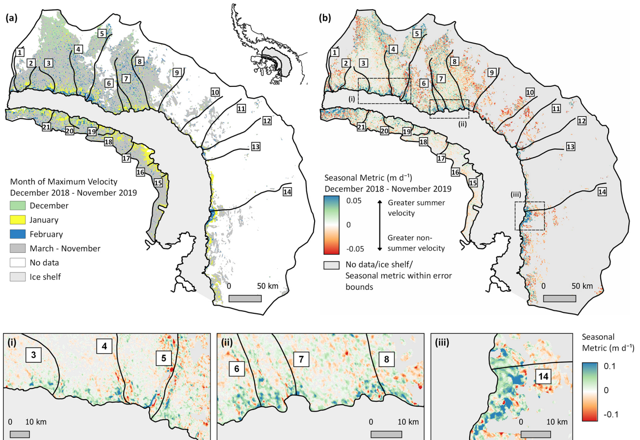
Figure 3. Spatially resolved patterns of seasonal ice flow as observed between December 2018 and November 2019. Panel (a) shows the month of maximum velocity ( v_{\text{time}} ) and (b) the calculated velocity anomaly ( v_{\text{anom}_{\text{SAR}}} ). In (b), positive velocity anomalies (blue) indicate summertime speed-up and negative (red) greater velocity during non-summertime months. Dashed boxes denote the location of the inset boxes (i–iii). See also Figs. B1–B4.
