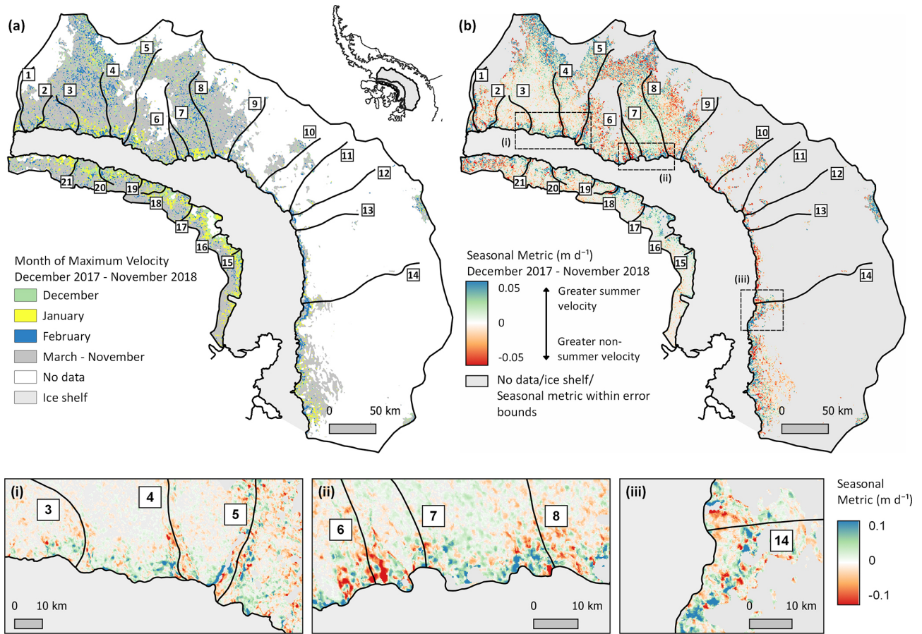
Figure B4. Same as Fig. 3 but showing spatially resolved patterns of seasonal ice flow as observed between December 2017 and November 2018. Panel (a) shows the month of maximum velocity ( v_{time} ) and (b) the calculated velocity anomaly ( v_{anomSAR} ). In (b), positive velocity anomalies (blue) indicate summertime speed-up and negative (red) greater velocity during non-summertime months. Dashed boxes denote the location of the inset boxes (i–iii). See also Figs. B1–B3.
