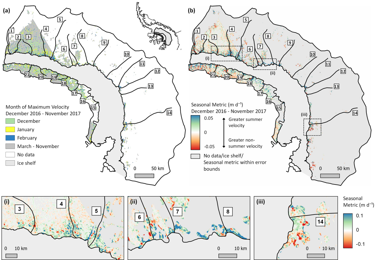
Figure B3. Same as Fig. 3 but showing spatially resolved patterns of seasonal ice flow as observed between December 2016 and November 2017. Panel (a) shows the month of maximum velocity ( v_{time} ) and (b) the calculated velocity anomaly ( v_{anomSAR} ). In (b), positive velocity anomalies (blue) indicate summertime speed-up and negative (red) greater velocity during non-summertime months. Dashed boxes denote the location of the inset boxes (i–iii). See also Figs. B1–B2 and B4.
