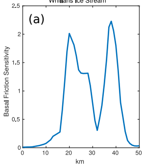
Whillans Ice Stream
