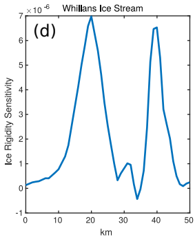
Whillans Ice Stream
