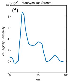
MacAyeal Ice Stream
