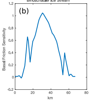
Bindschadler Ice Stream
