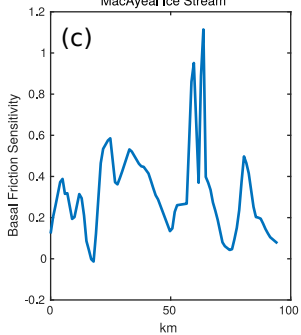
MacAyeal Ice Stream
