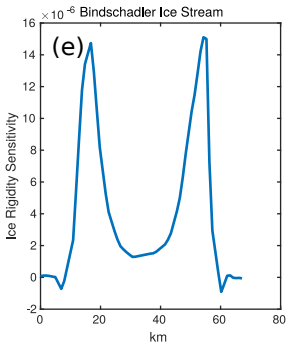
Bindschadler Ice Stream
