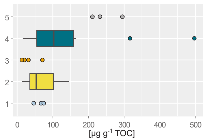
Branched and cyclic alkanes
