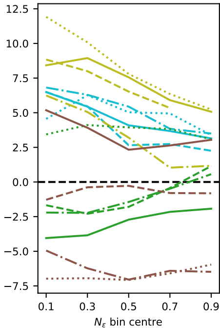
(a) T_a
