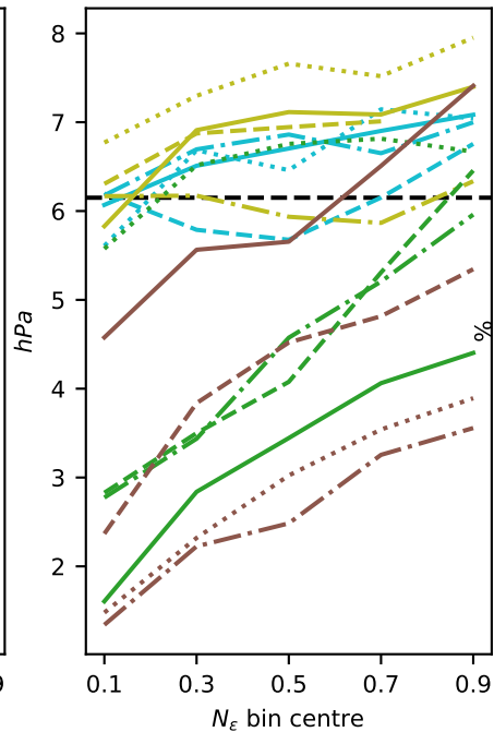
(c) e_a
