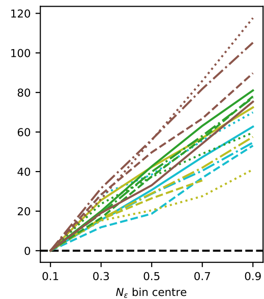
(e) LWnet cloud effect
