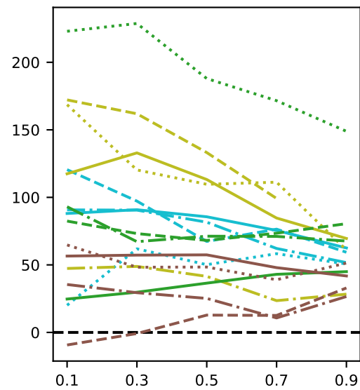
(f) Rnet cloud effect
