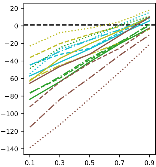
(e) LWnet cloud effect
