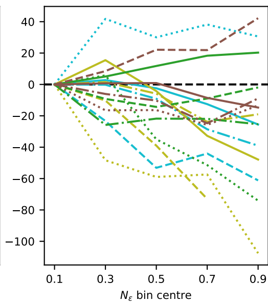
(f) Rnet cloud effect
