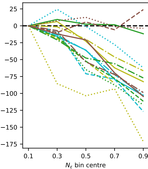
(f) SWin + LWin cloud effect
