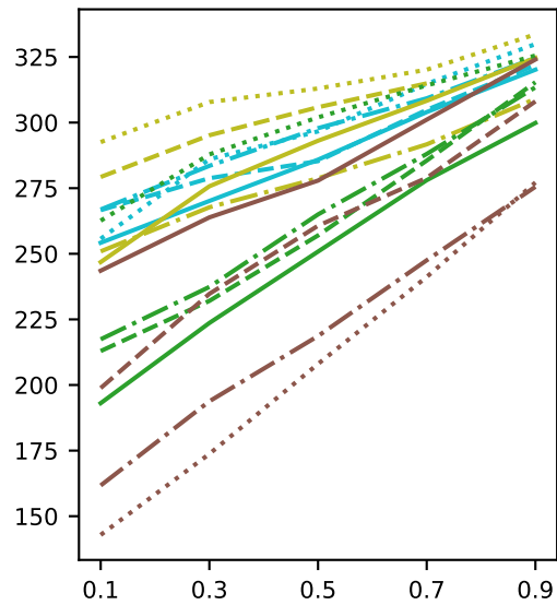
(e) LWin cloud effect
