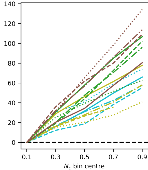
(e) LWin cloud effect
