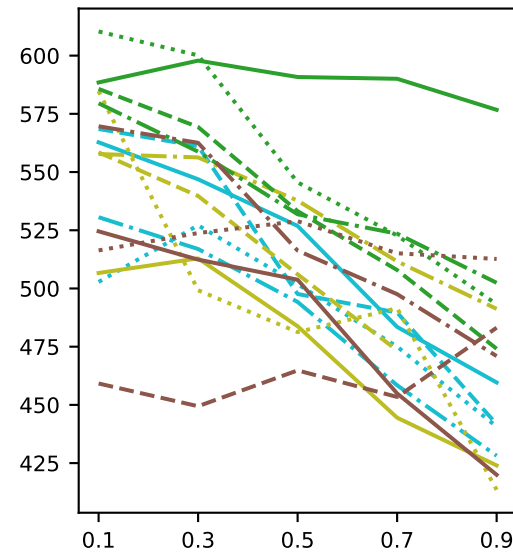
(f) SWin + LWin cloud effect
