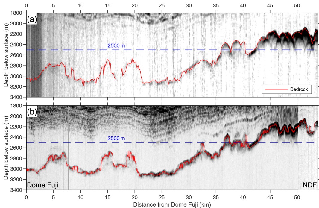
Figure 2. Radargrams between Dome Fuji and NDF acquired by the radar systems used in (a) JARE54 (2012/13) with 3-element Yagi antenna and (b) JARE59 (2017/18) with 11-element Yagi antenna. The lines indicate bedrock topography traced from the radar data. Note that radargrams shown in (b) were generated by data acquired on 17 and 21 December 2017. The colour range in radargrams (a) and (b) is 1.25–1.80 and -110 – 0 dBm, respectively.
