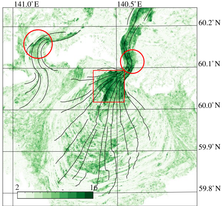
(b) signal-to-noise
