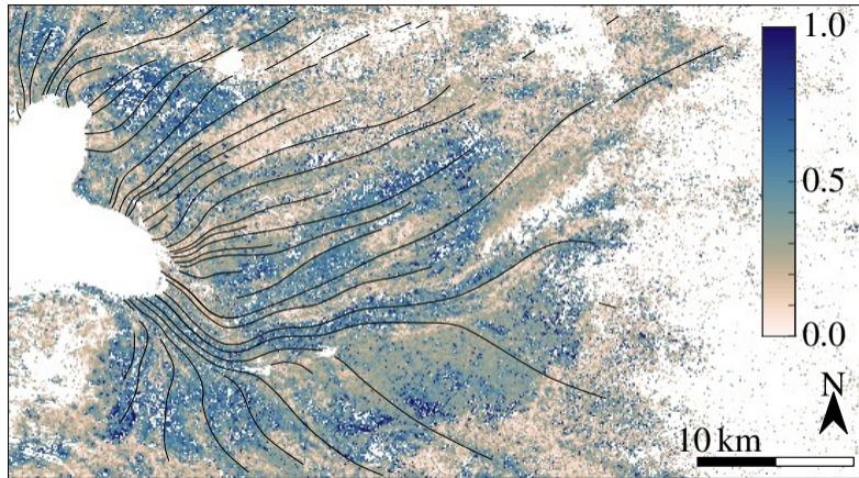
(a) elongation of correlation surface
