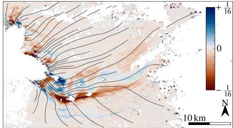
(b) estimated surface shear
