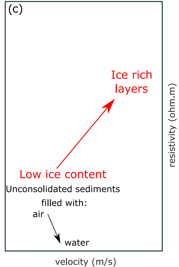
Qualitative geophysical signature
