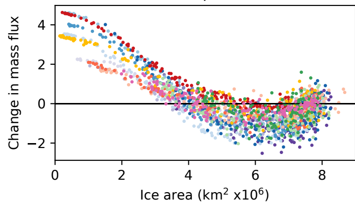
(c) Top melt
