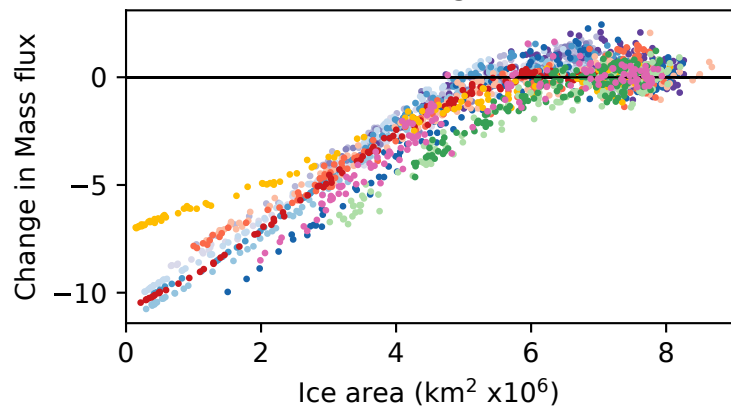
(b) Basal growth
