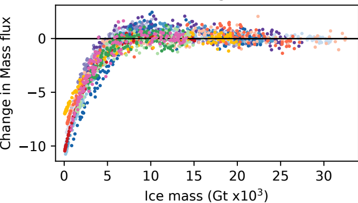
(a) Basal growth
