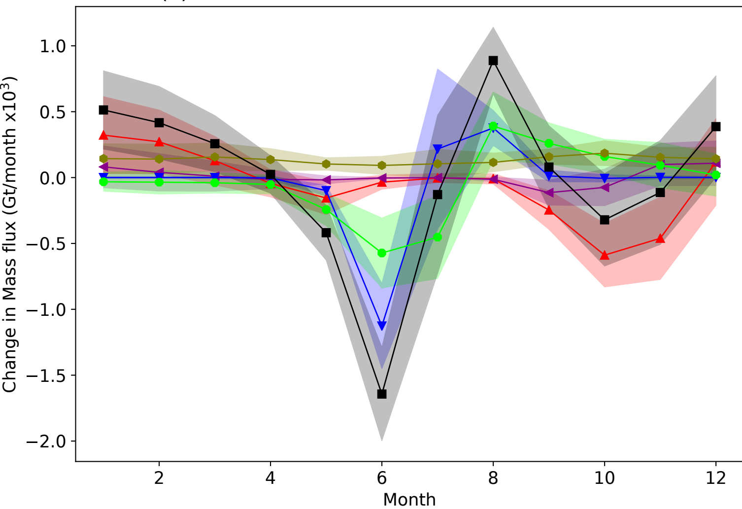
(b) Multi-model mean: 2040-49 minus 1960-89
