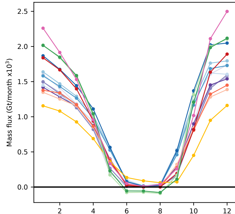
(c) Top melt
