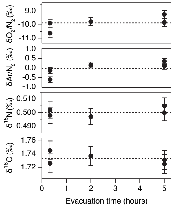
(a) Bubbly ice (446.4 m)
