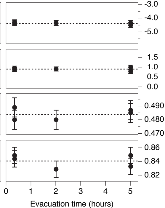
(b) Clathrate hydrate ice (2001.1 m)
