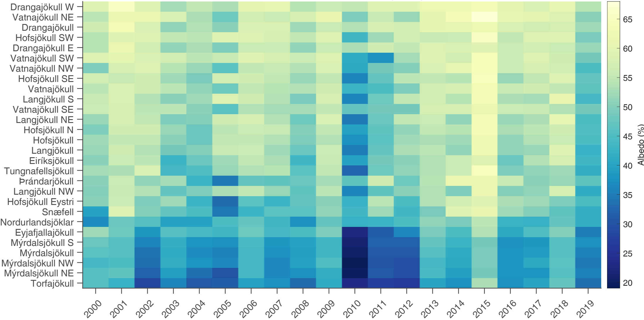
Melt Season Mean Albedo (MJJA)
