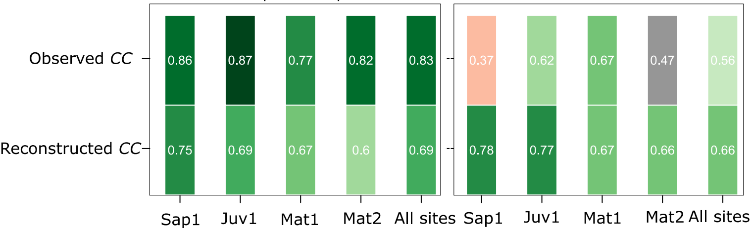
Air temperature
