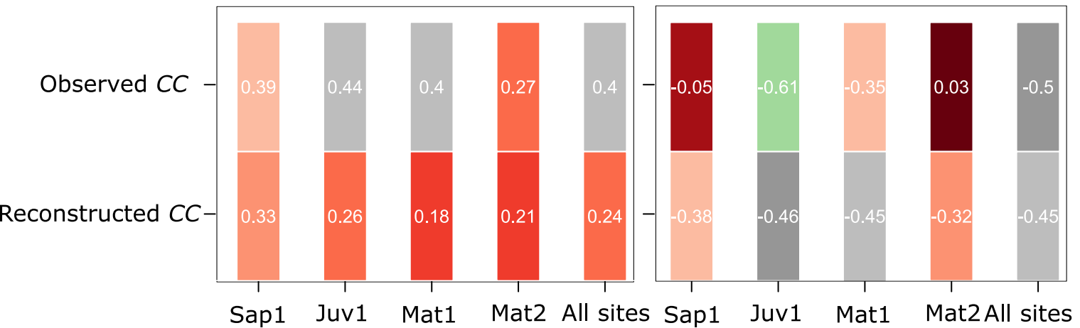
Snow density
