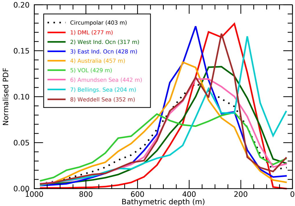
Normalised PDF of fast ice formation depth
