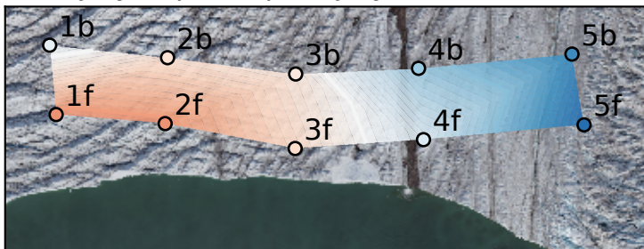
(b) speedup 14 July - calving 20 July
