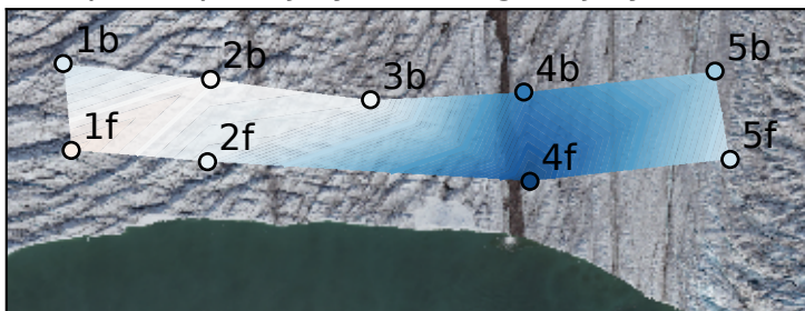
(c) calving 20 July - GPS retrieval 22 July
