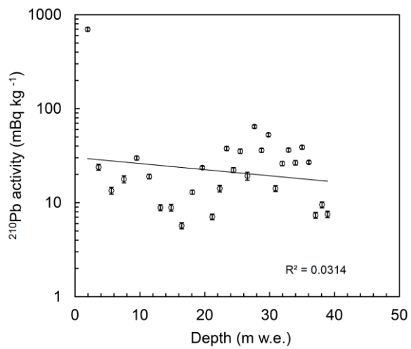
Figure S2. ADA16 profile of ^{210}\text{Pb} activity concentrations.
