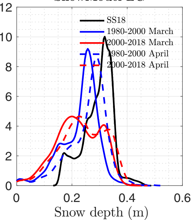
SnowModel-LG
