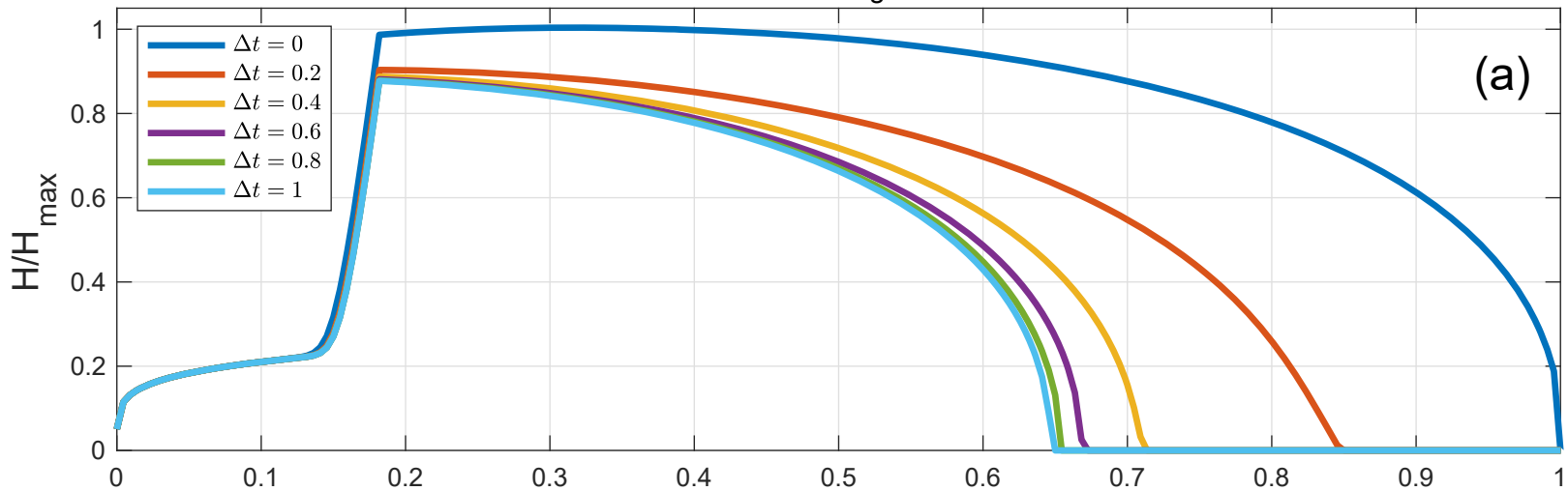
Debris-free glacier
