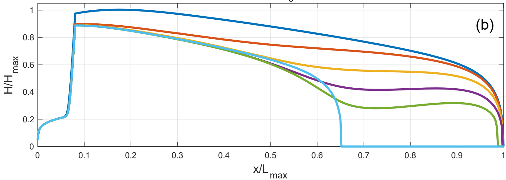
Debris-covered glacier
