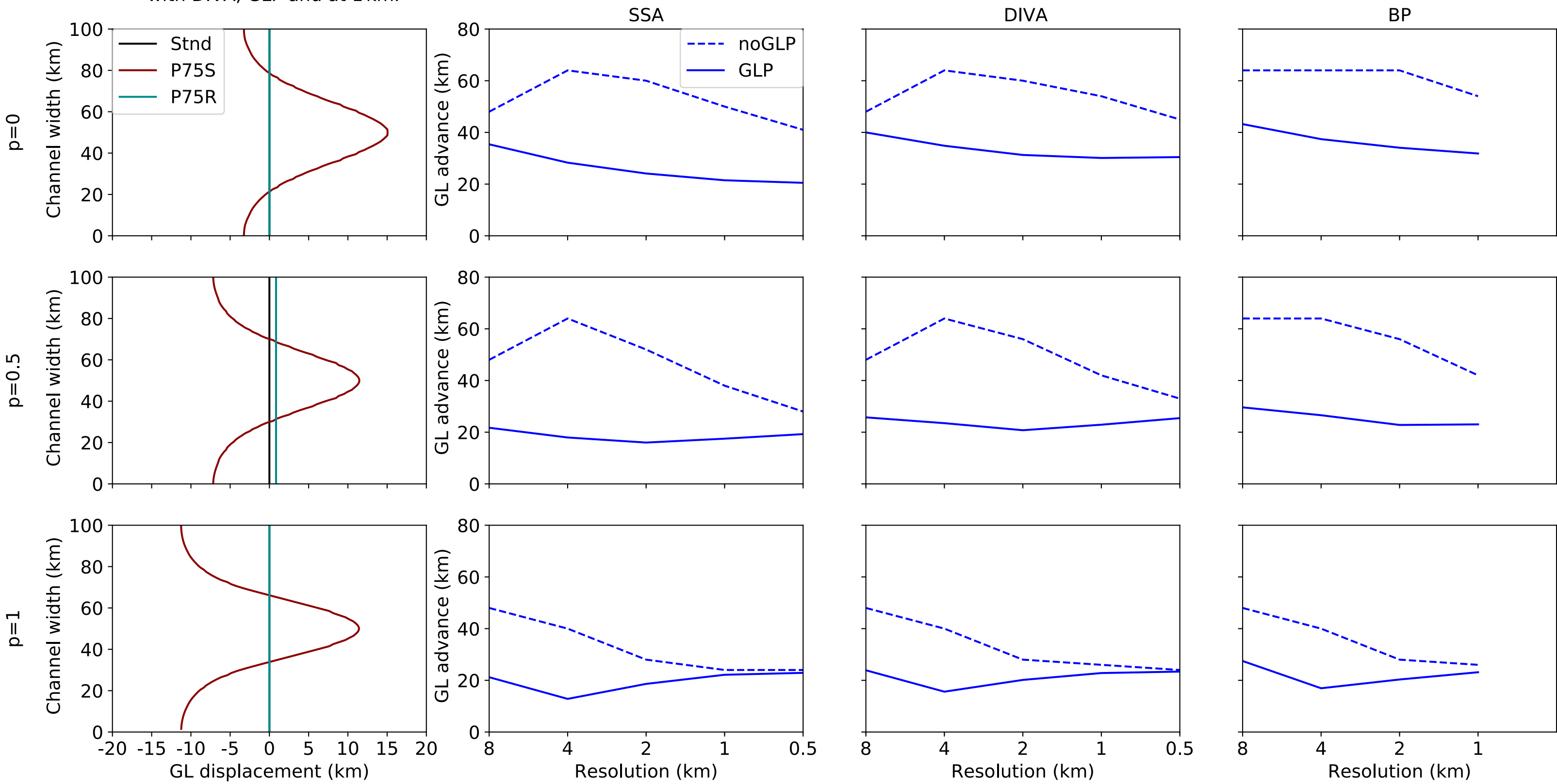
Full set of MISMIP3d experiments with DIVA, GLP and at 1 km.
