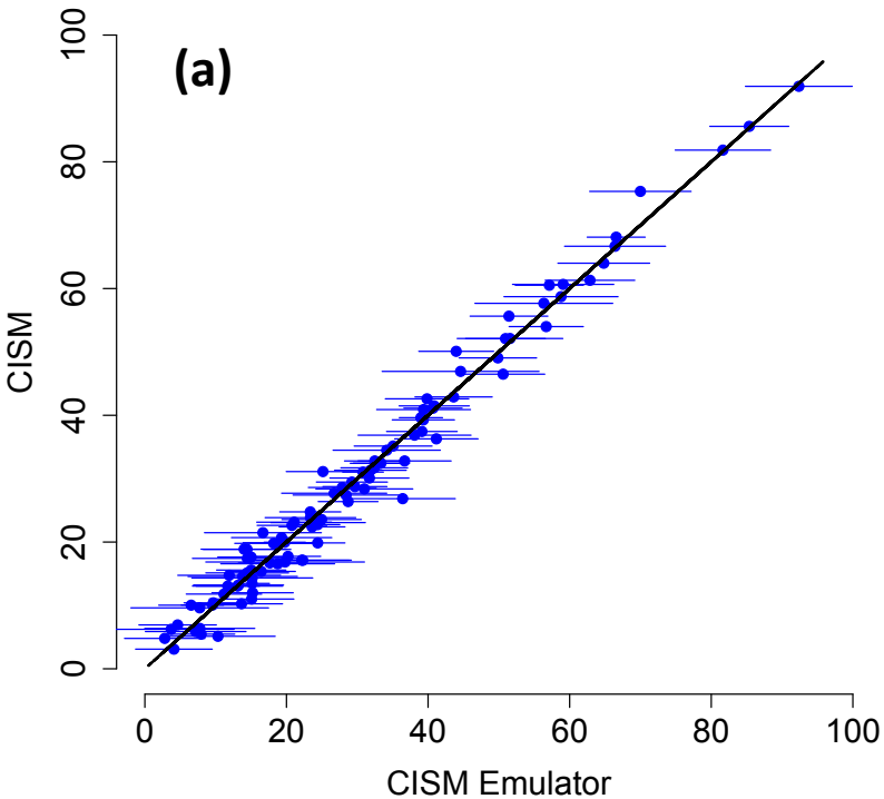
SLR (mm) emulator validation at year 100
