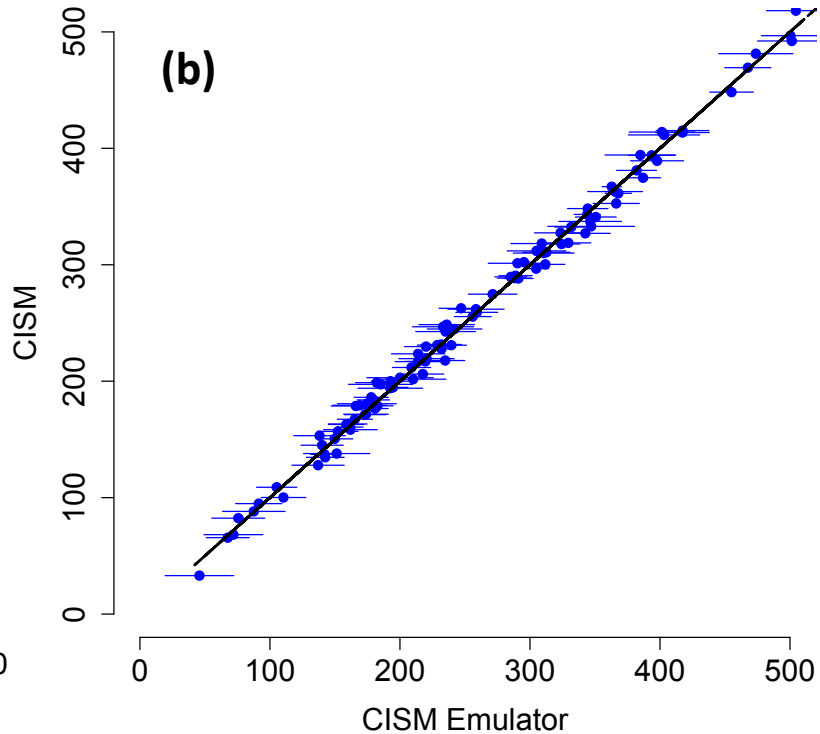
SLR (mm) emulator validation at year 200
