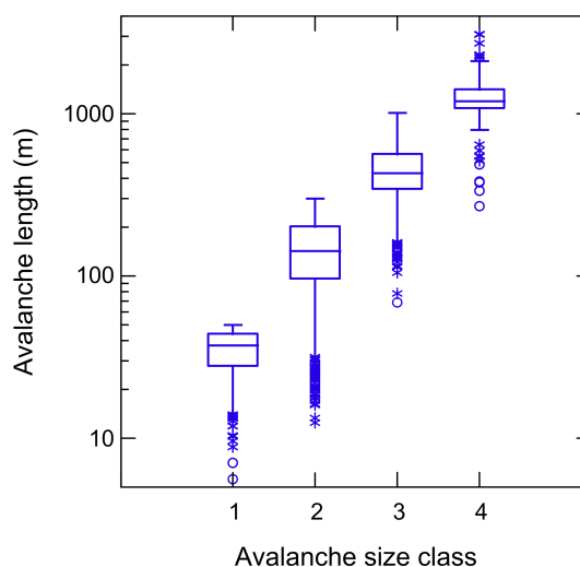
Figure 1. Distribution of avalanche length per avalanche size class for the 21-year data set of avalanche observations from the region of Davos applying the classification criteria given in Table 1. Boxes span the interquartile range from the first to third quartiles with a horizontal line showing the median. Whiskers show the range of observed values that fall within 1.5 times the interquartile range above the third and below the first quartiles. Asterisks and open circles refer to outliers and far outliers beyond the fences. Numbers indicate avalanches per class; total number of avalanches: N = 13\,802 .
