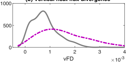
(b) Vertical heat flux divergence
