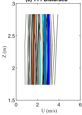
(c) TT1 Disturbed
