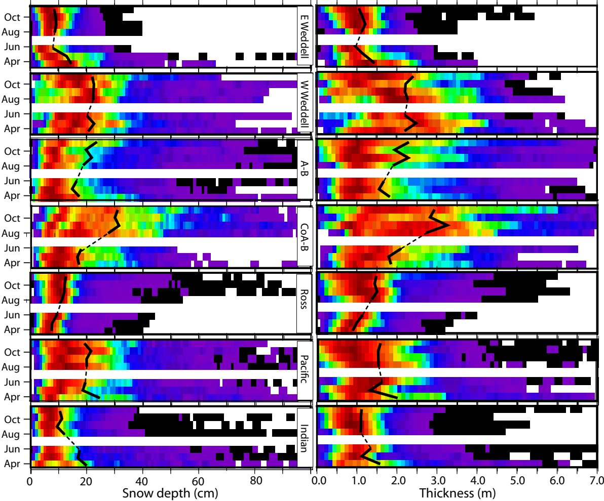
(a) Snow depth
