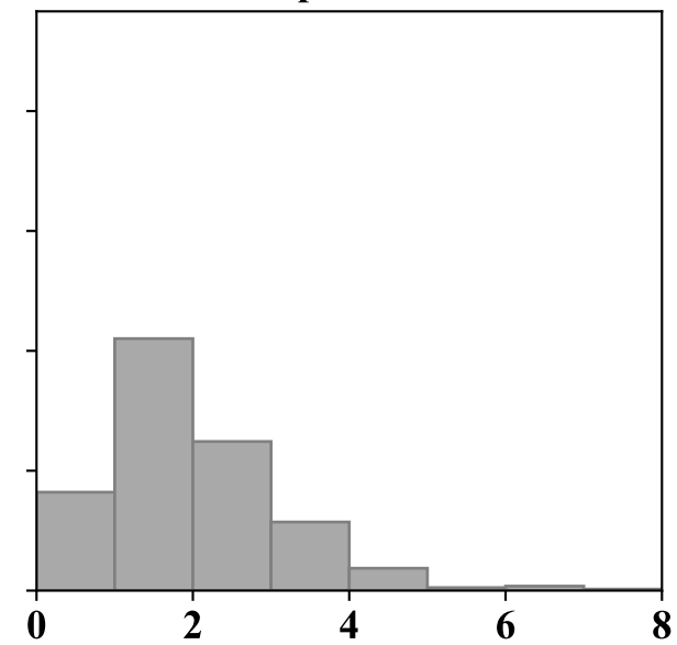
Depth hoar
