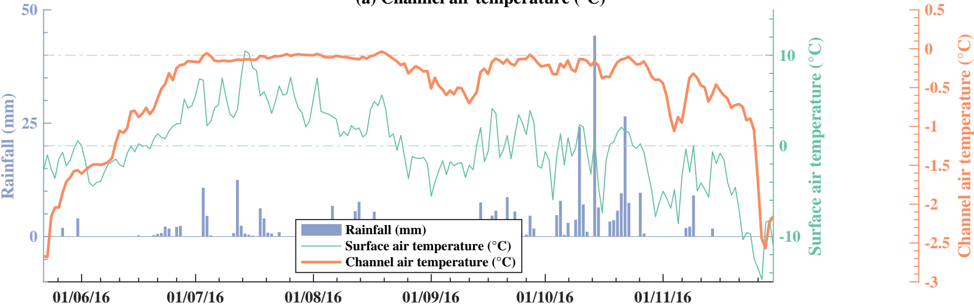
(a) Channel air temperature (°C)
