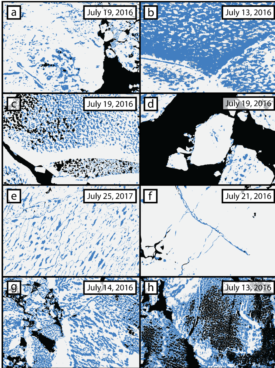
Figure S1. Classified versions of the images shown in Figure 10. White regions are snow/ice, blue regions are melt ponds or submerged ice, and black regions are open water.
