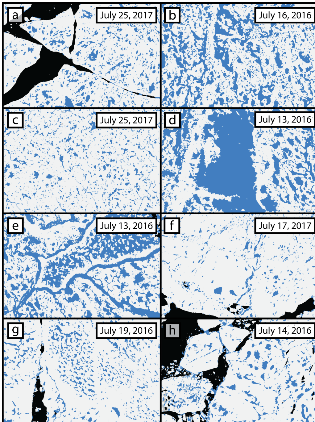
Figure S2. Classified versions of the images shown in Figure 11. White regions are snow/ice, blue regions are melt ponds or submerged ice, black regions are open water.
