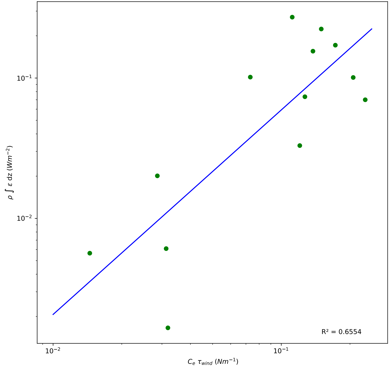
Integrated TKE dissipation rate as a function of wind stress
