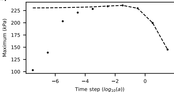
(b) Greatest principal stress
