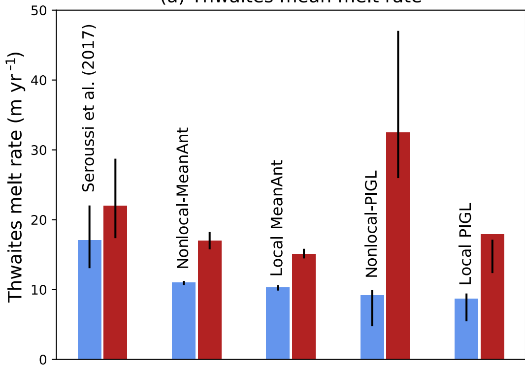
(a) Thwaites mean melt rate
