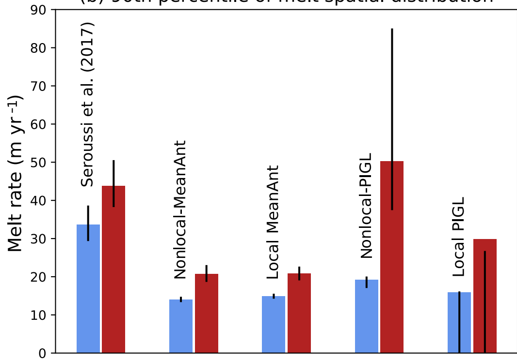
(b) 90th percentile of melt spatial distribution
